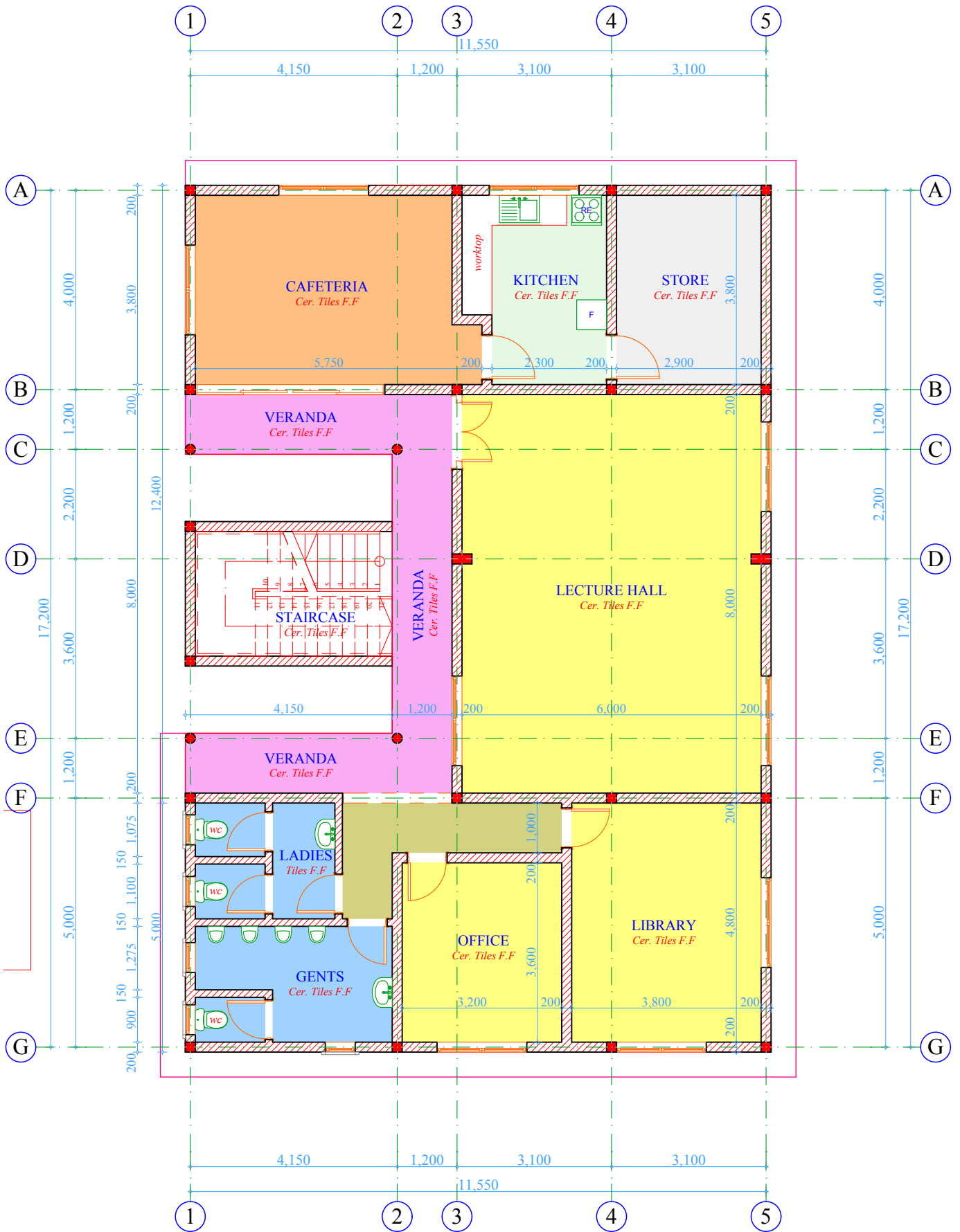
GROUND FLOOR PLAN Scale:1:105
